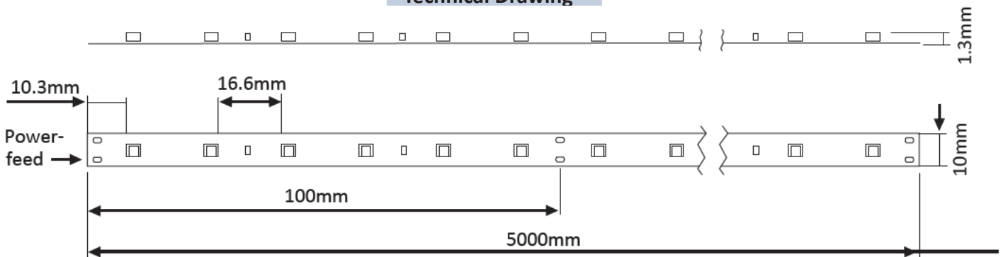
Technical Drawing
